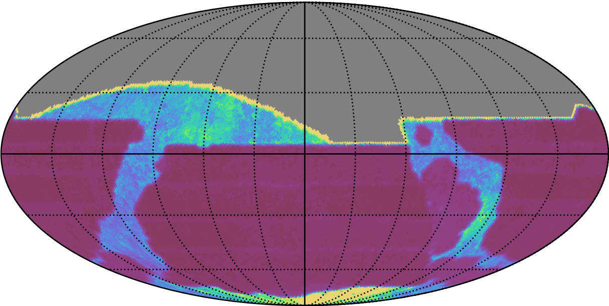
ddf_acor_sf10_lsf15_lsr20_v3.4_10yrs All sky all bands: Median Inter-Night Gap
