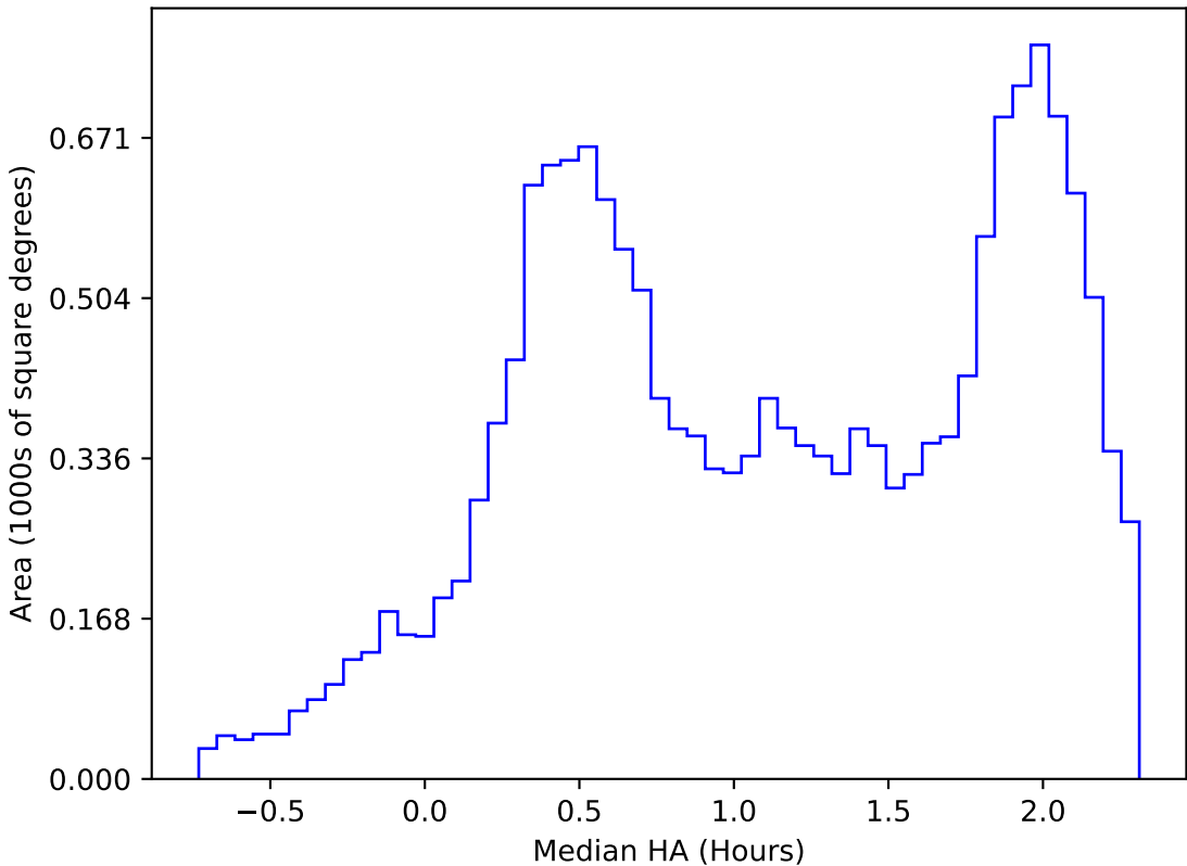
ddf_acor_sf10_lsf15_lsr20_v3.4_10yrs WFD z band: Median HA
