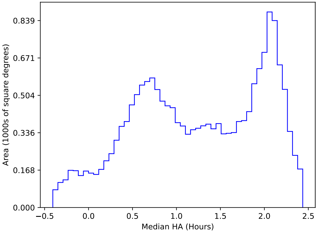
ddf_acor_sf10_lsf15_lsr20_v3.4_10yrs WFD y band: Median HA
