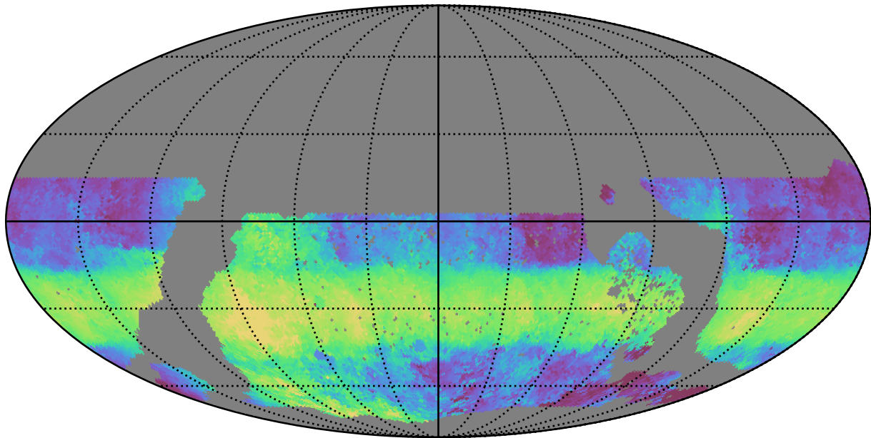
ddf_acor_sf10_lsf15_lsr20_v3.4_10yrs WFD u band: Median HA
