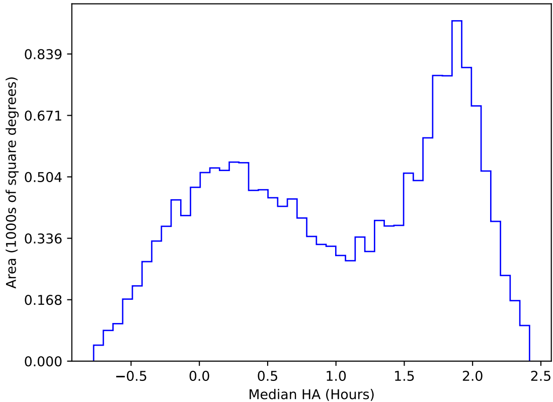
ddf_acor_sf10_lsf15_lsr20_v3.4_10yrs WFD u band: Median HA
