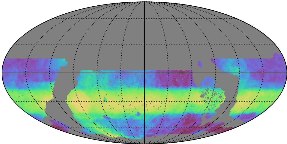
ddf_acor_sf10_lsf15_lsr20_v3.4_10yrs WFD r band: Median HA
