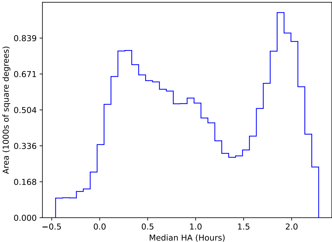
ddf_acor_sf10_lsf15_lsr20_v3.4_10yrs WFD i band: Median HA
