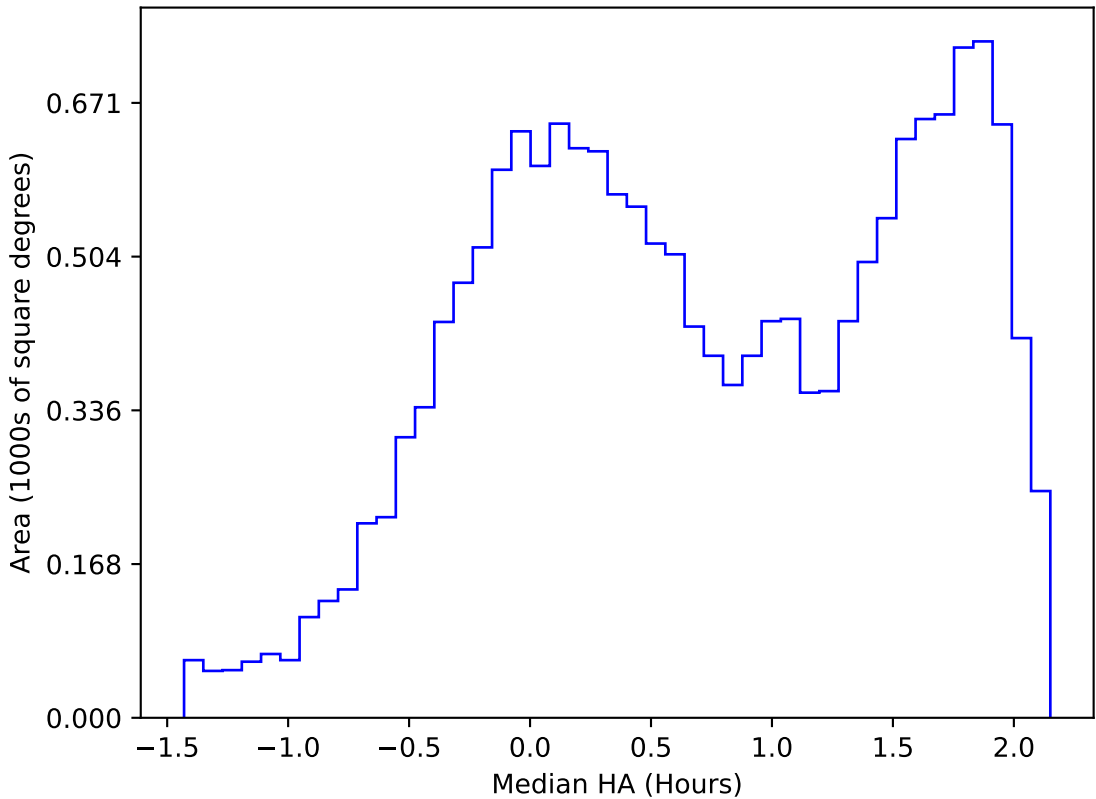
ddf_acor_sf10_lsf15_lsr20_v3.4_10yrs WFD g band: Median HA
