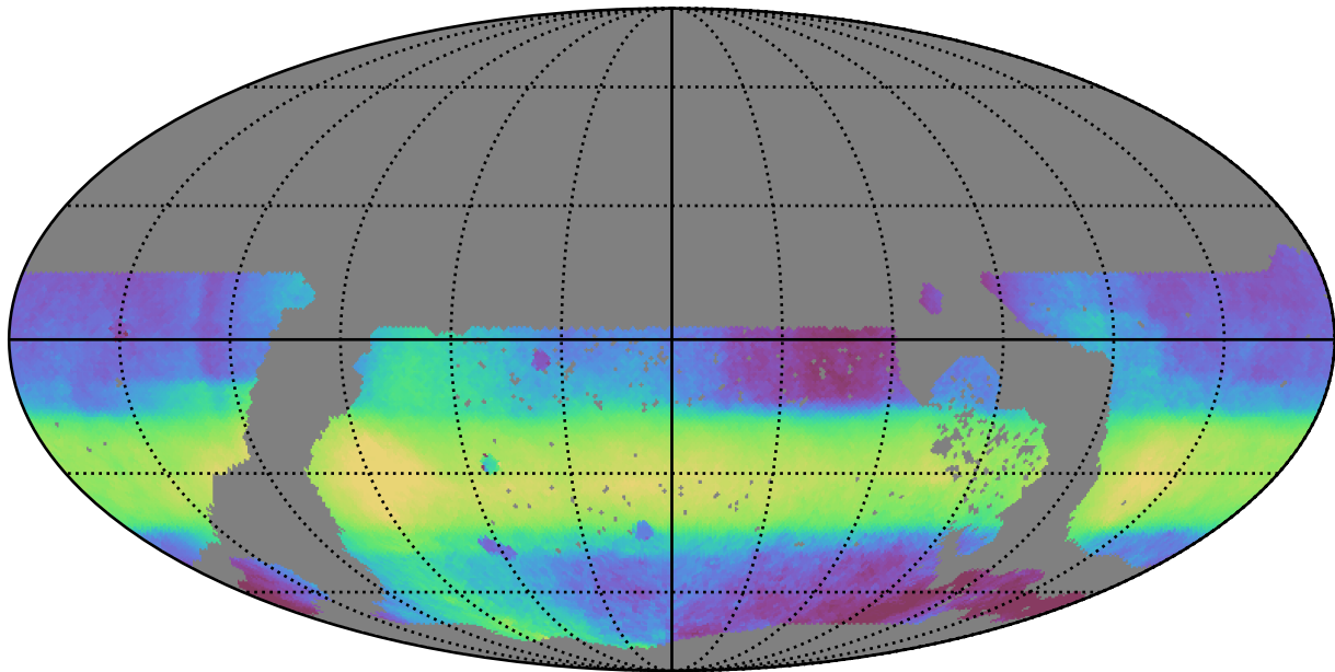
ddf_acor_sf10_lsf15_lsr20_v3.4_10yrs WFD all bands: Median HA
