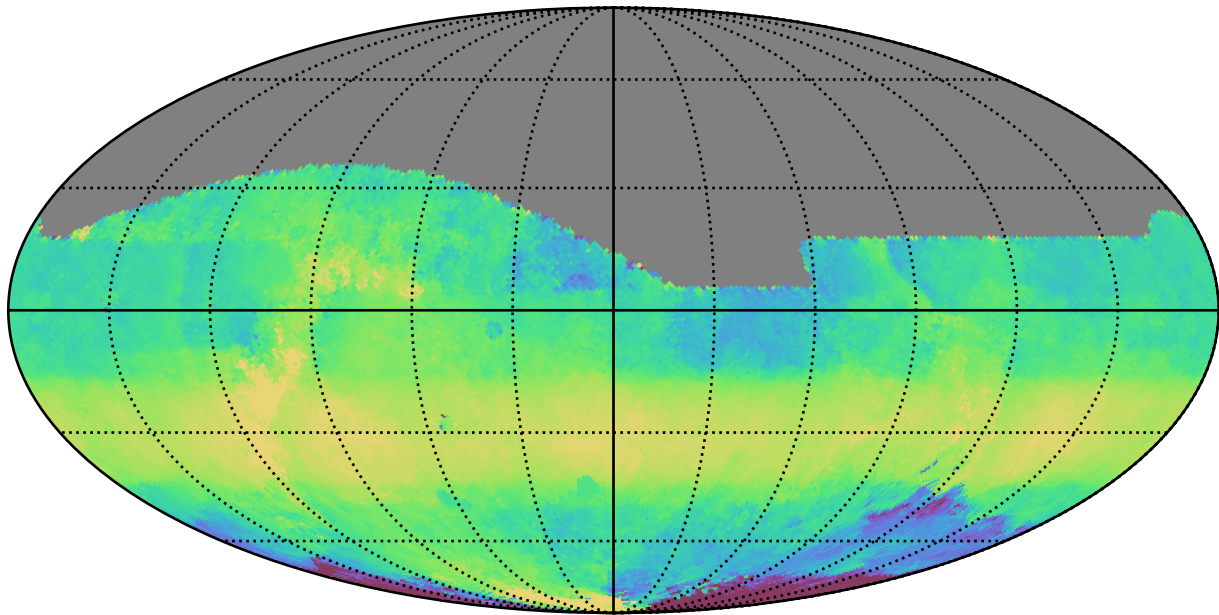
ddf_acor_sf10_lsf15_lsr20_v3.4_10yrs All sky z band: Median HA
