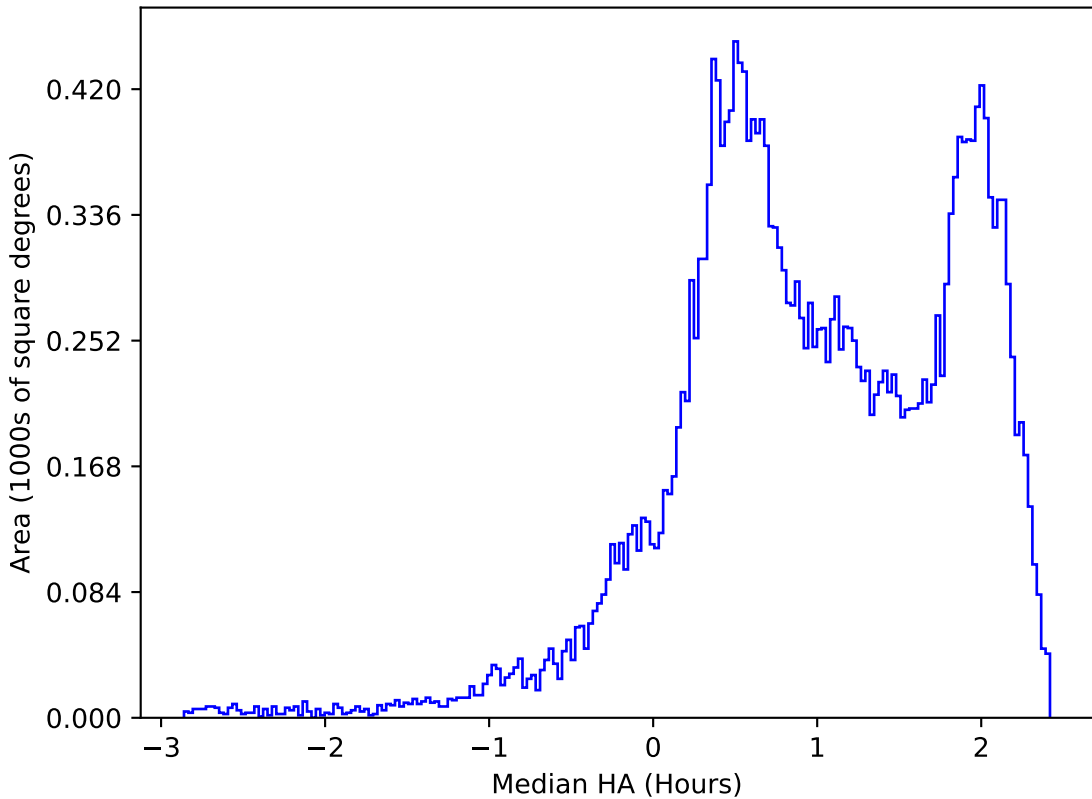
ddf_acor_sf10_lsf15_lsr20_v3.4_10yrs All sky z band: Median HA
