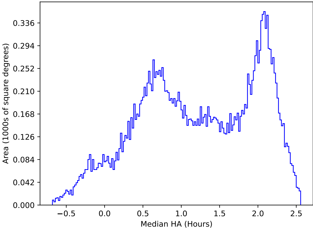
ddf_acor_sf10_ls15_lsr20_v3.4_10yrs All sky y band: Median HA
