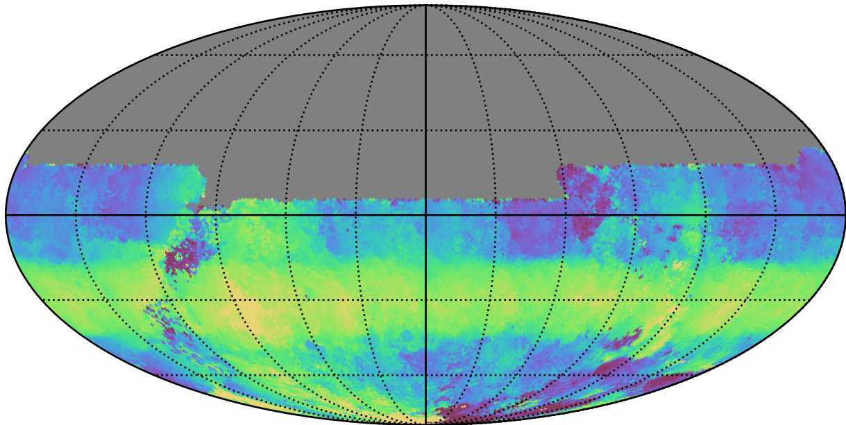
ddf_acor_sf10_lsf15_lsr20_v3.4_10yrs All sky u band: Median HA
