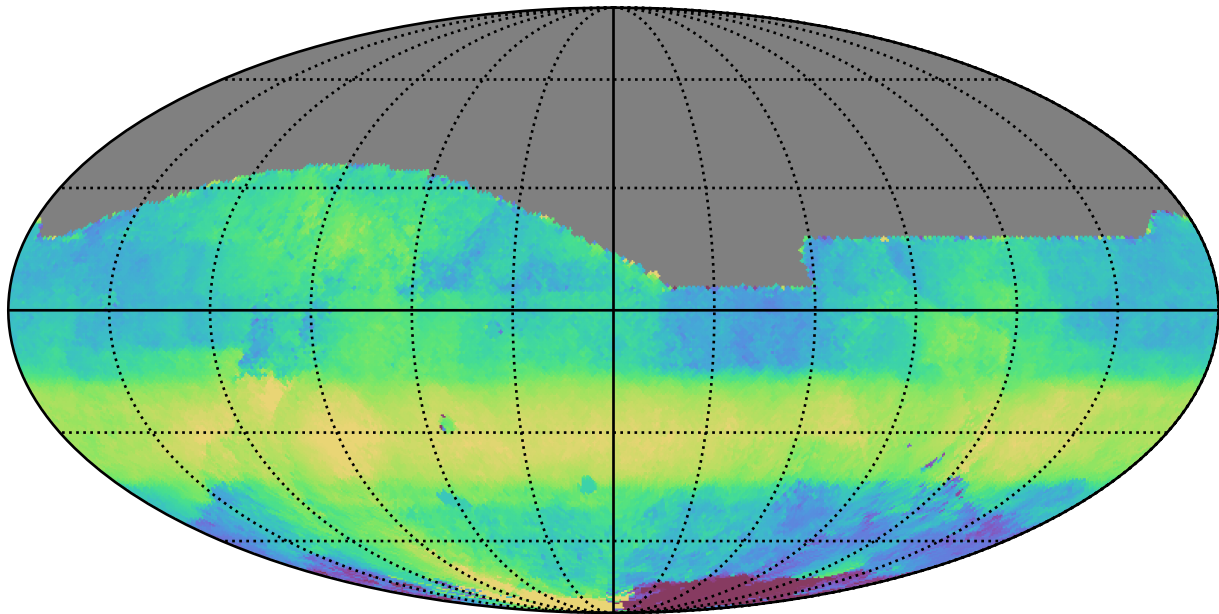
ddf_acor_sf10_lsf15_lsr20_v3.4_10yrs All sky r band: Median HA
