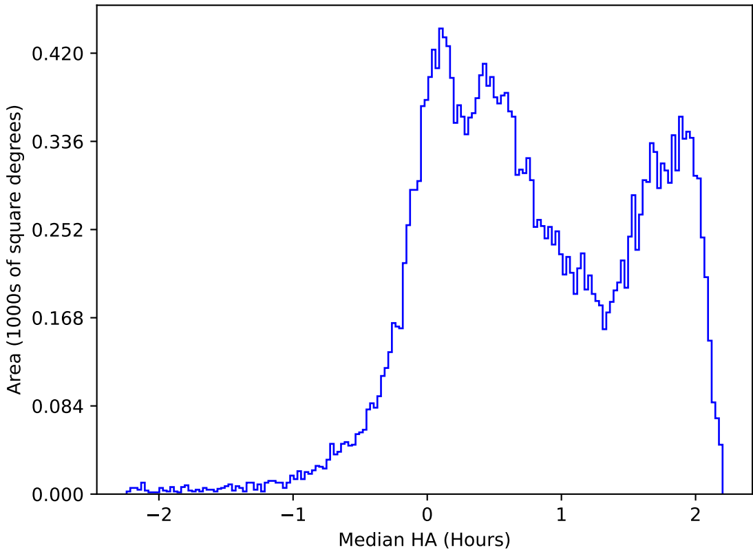
ddf_acor_sf10_lsf15_lsr20_v3.4_10yrs All sky r band: Median HA
