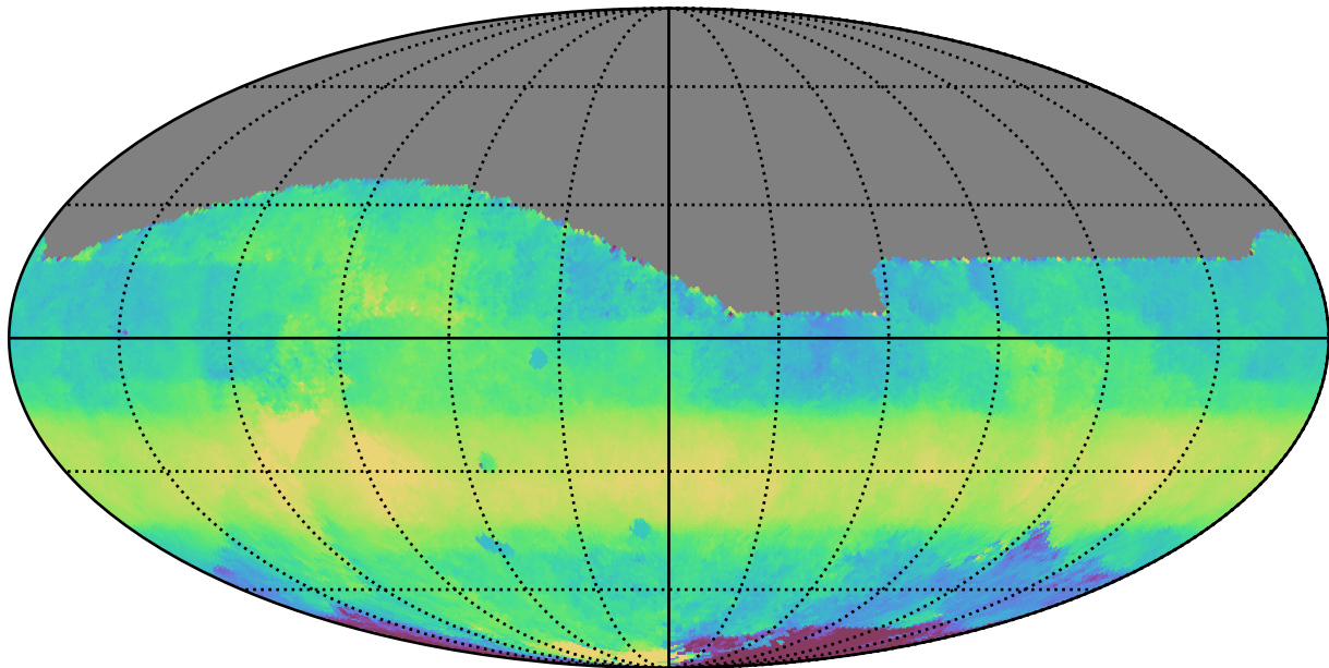
ddf_acor_sf10_lsf15_lsr20_v3.4_10yrs All sky i band: Median HA
