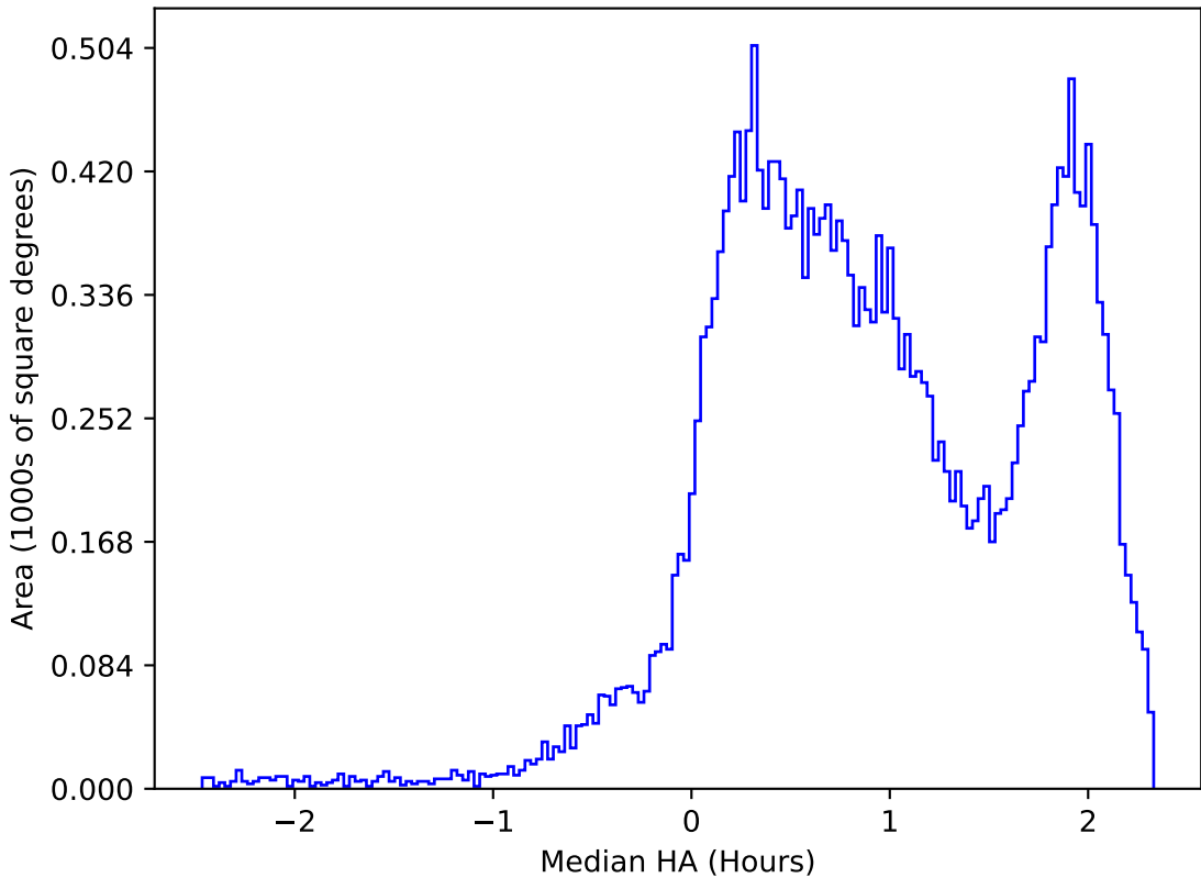
ddf_acor_sf10_lsf15_lsr20_v3.4_10yrs All sky i band: Median HA
