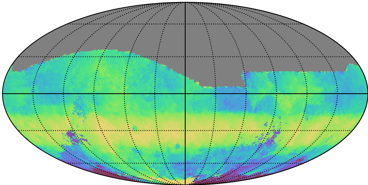
ddf_acor_sf10_lsf15_lsr20_v3.4_10yrs All sky g band: Median HA
