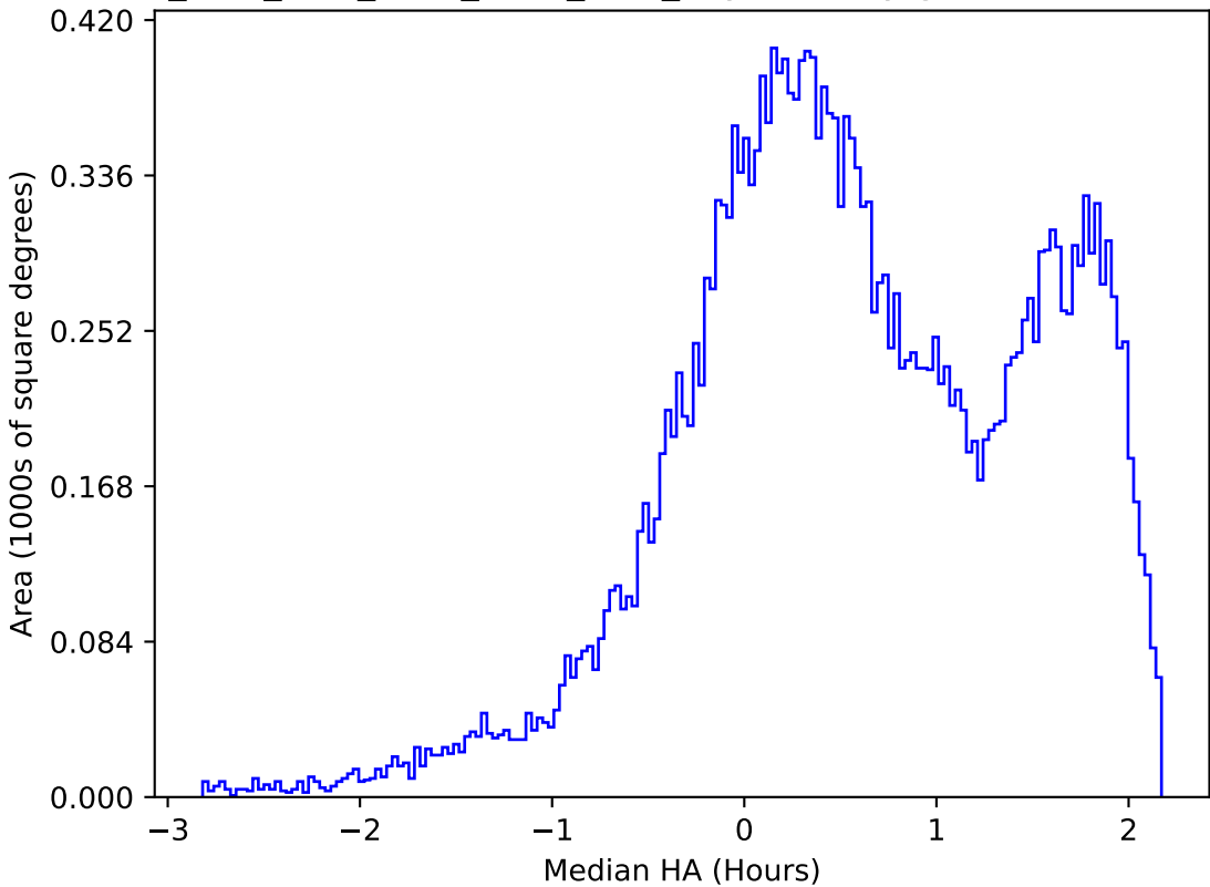
ddf_acor_sf10_ls15_lsr20_v3.4_10yrs All sky g band: Median HA
