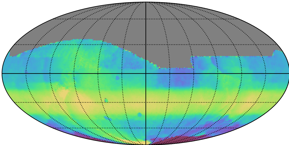
ddf_acor_sf10_lsf15_lsr20_v3.4_10yrs All sky all bands: Median HA
