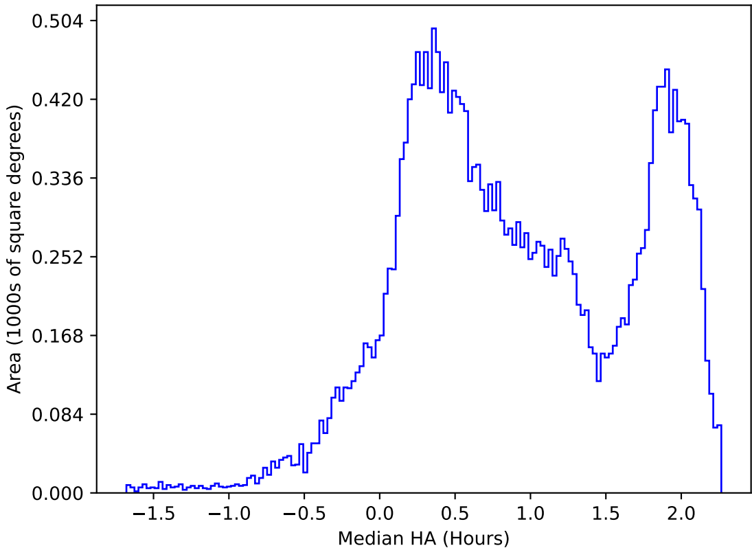
ddf_acor_sf10_lsf15_lsr20_v3.4_10yrs All sky all bands: Median HA
