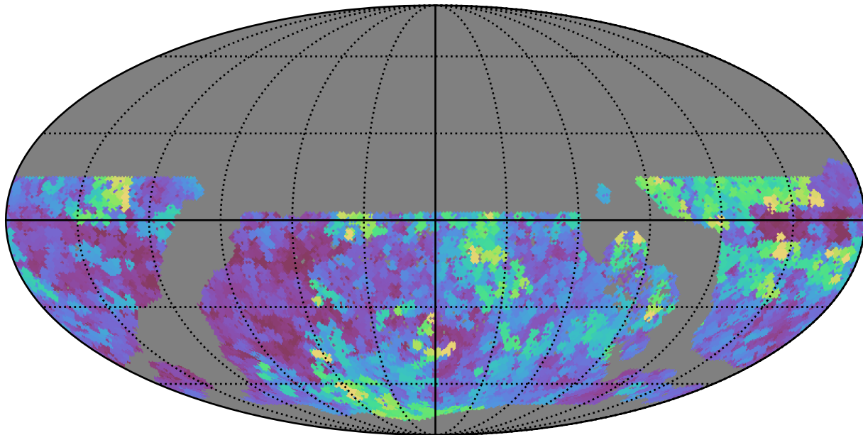
ddf_acor_sf10_lsf15_lsr20_v3.4_10yrs WFD g band: Max seeingEff
