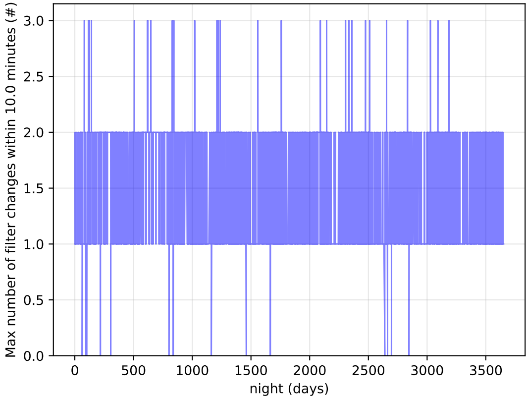
ddf_acor_sf10_Isf15_Isr20_v3.4_10yrs Per Night: Max number of filter changes within 10.0 minutes
