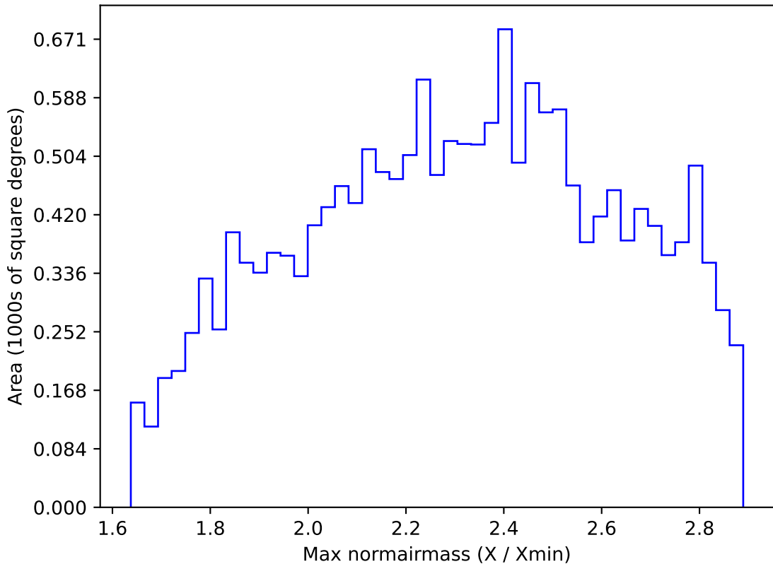
ddf_acor_sf10_lsf15_lsr20_v3.4_10yrs WFD z band: Max normairmass
