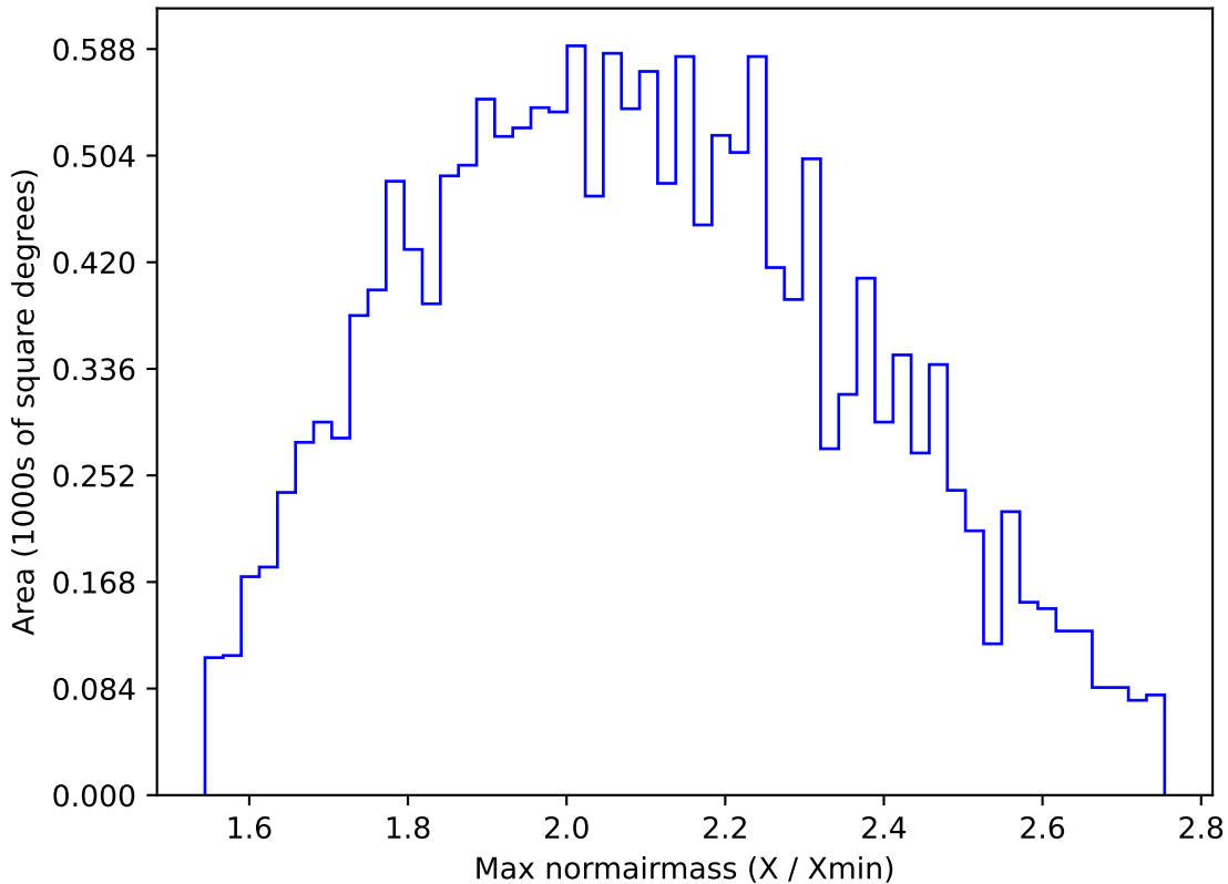
ddf_acor_sf10_lsf15_lsr20_v3.4_10yrs WFD y band: Max normairmass
