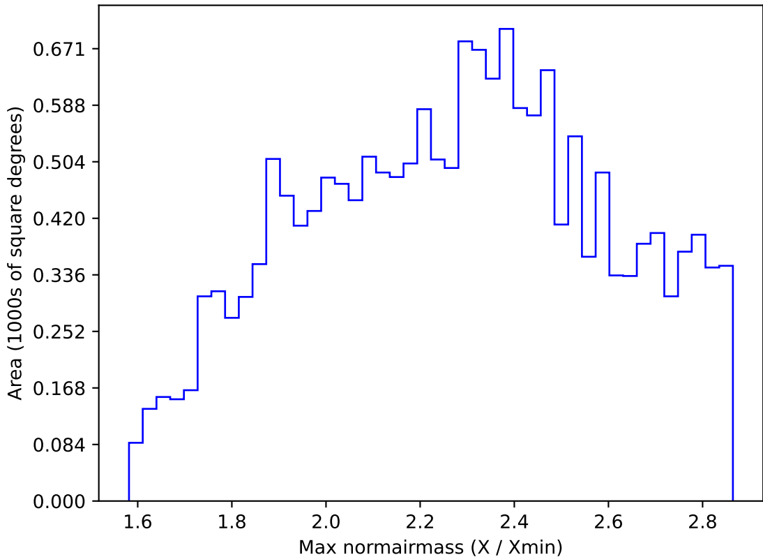
ddf_acor_sf10_lsf15_lsr20_v3.4_10yrs WFD i band: Max normairmass
