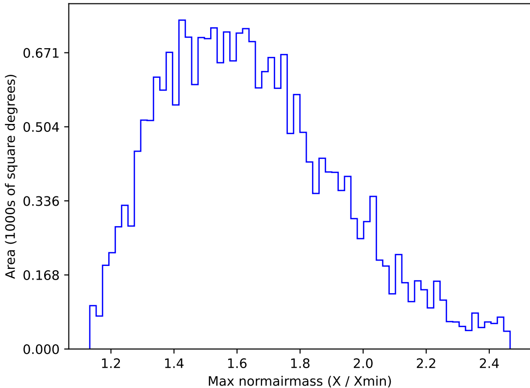
ddf_acor_sf10_lsf15_lsr20_v3.4_10yrs All sky u band: Max normairmass
