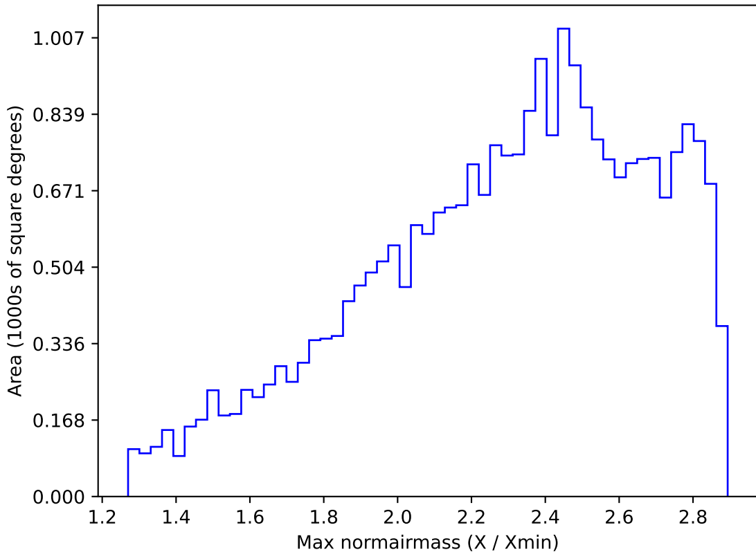
ddf_acor_sf10_lsf15_lsr20_v3.4_10yrs All sky all bands: Max normairmass
