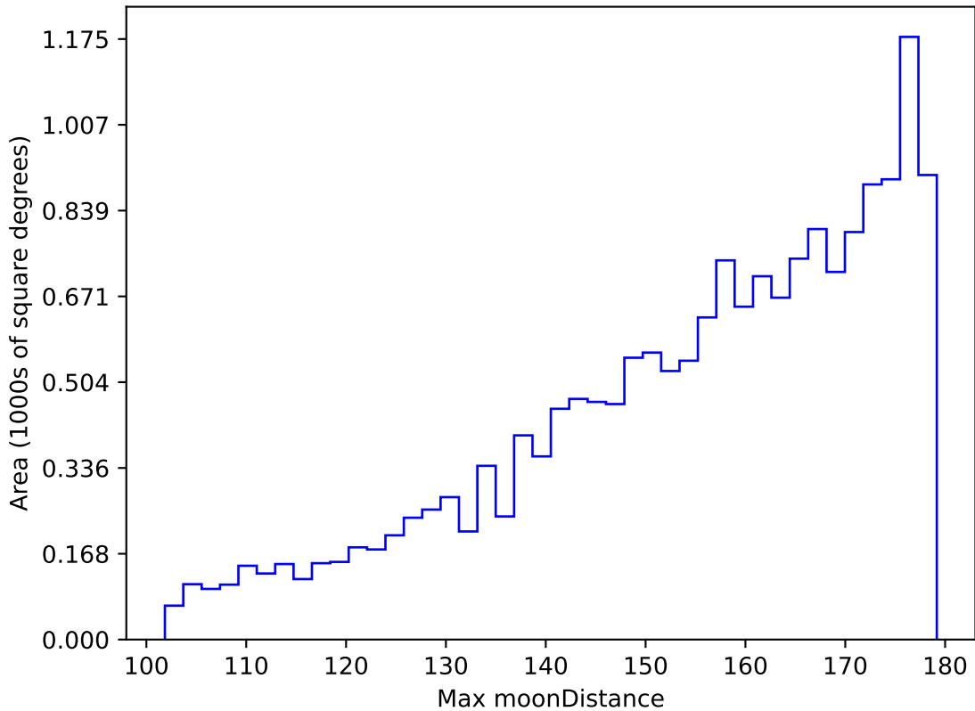
ddf_acor_sf10_ls15_lsr20_v3.4_10yrs WFD u band: Max moonDistance
