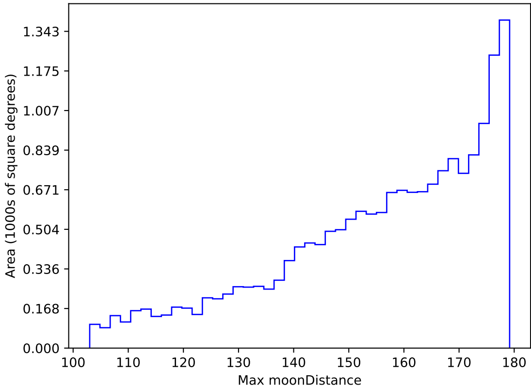
ddf_acor_sf10_lsf15_lsr20_v3.4_10yrs WFD i band: Max moonDistance
