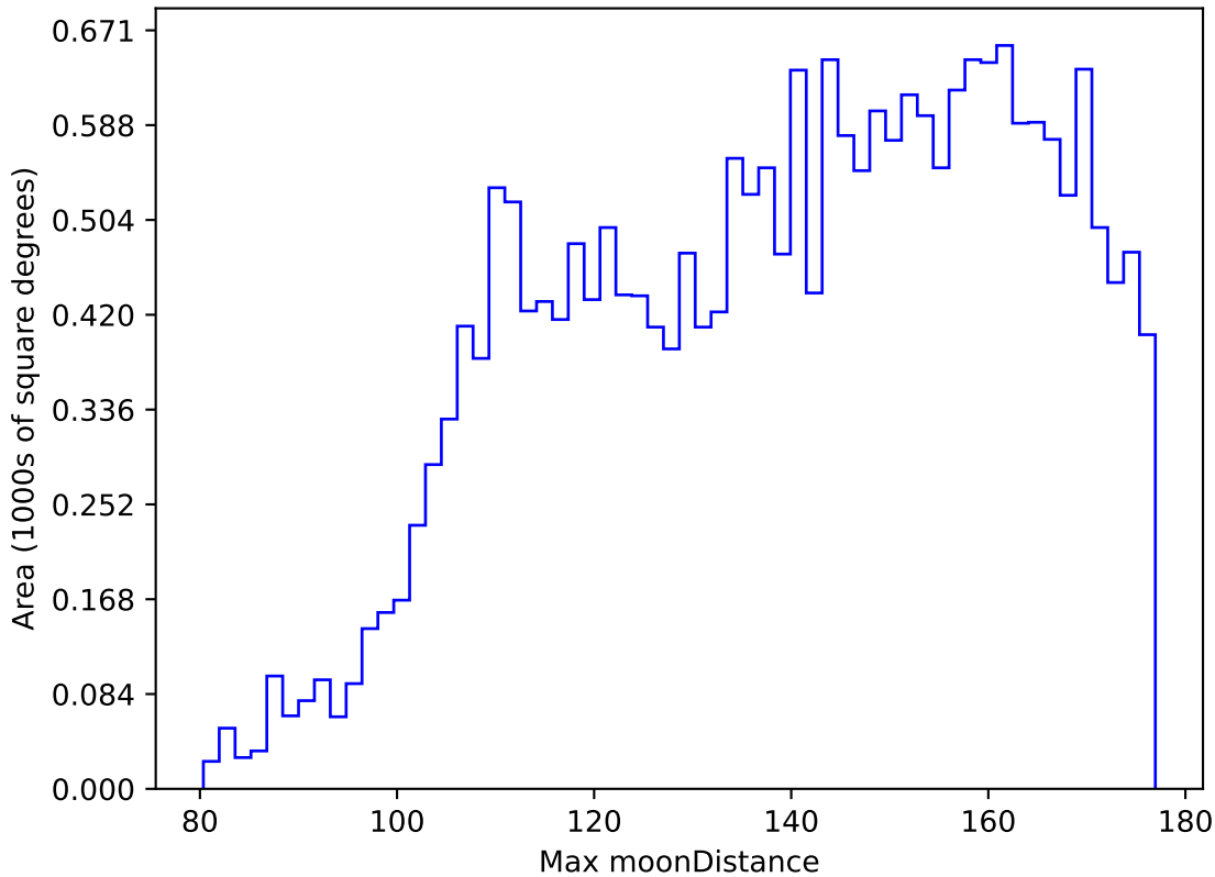
ddf_acor_sf10_lsf15_lsr20_v3.4_10yrs All sky y band: Max moonDistance
