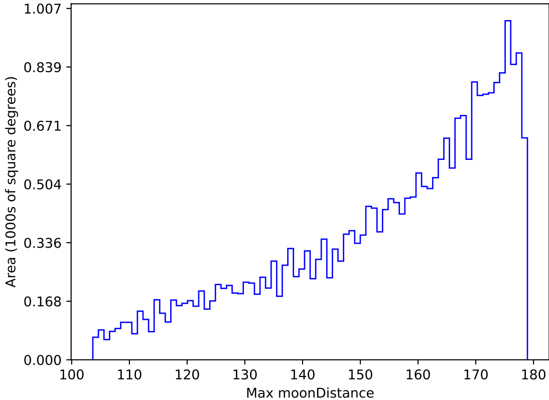
ddf_acor_sf10_lsf15_lsr20_v3.4_10yrs All sky g band: Max moonDistance
