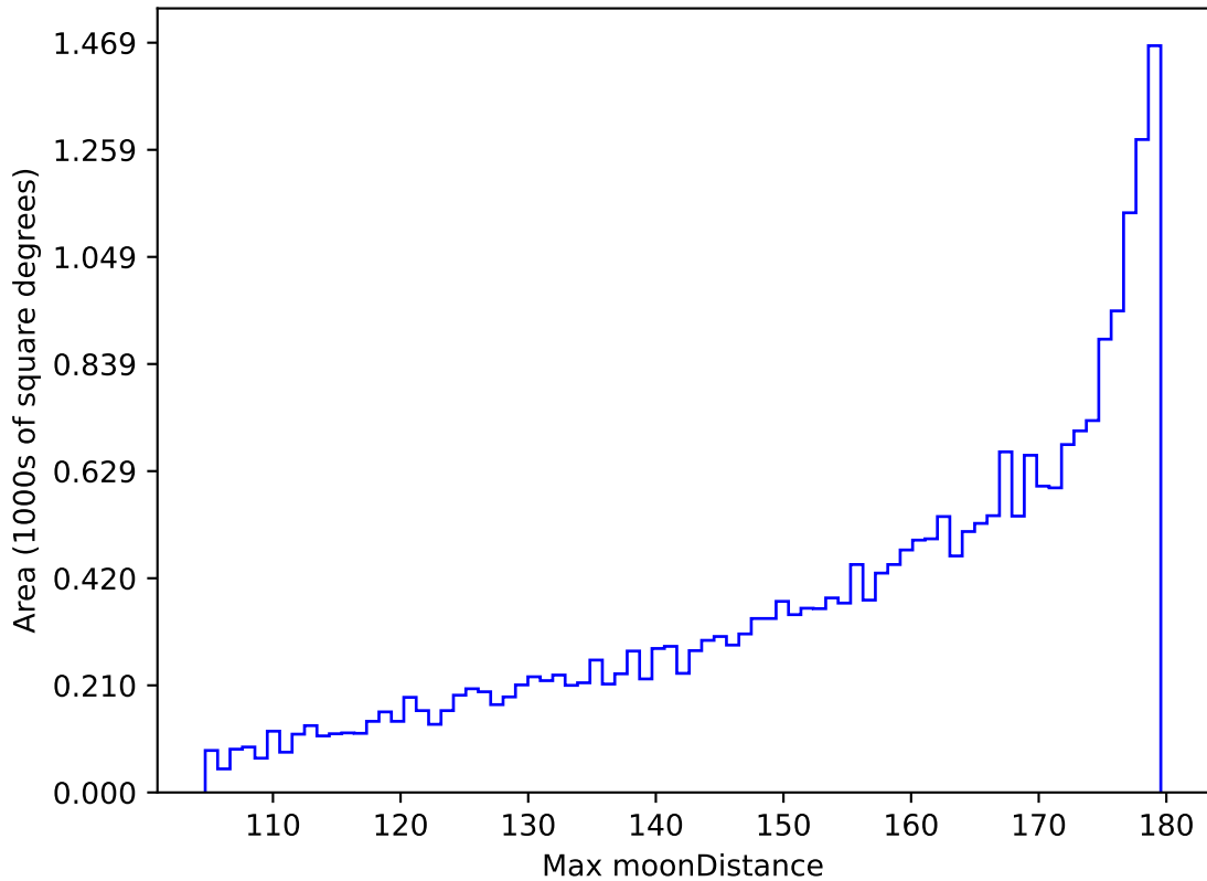
ddf_acor_sf10_lsf15_lsr20_v3.4_10yrs All sky all bands: Max moonDistance
