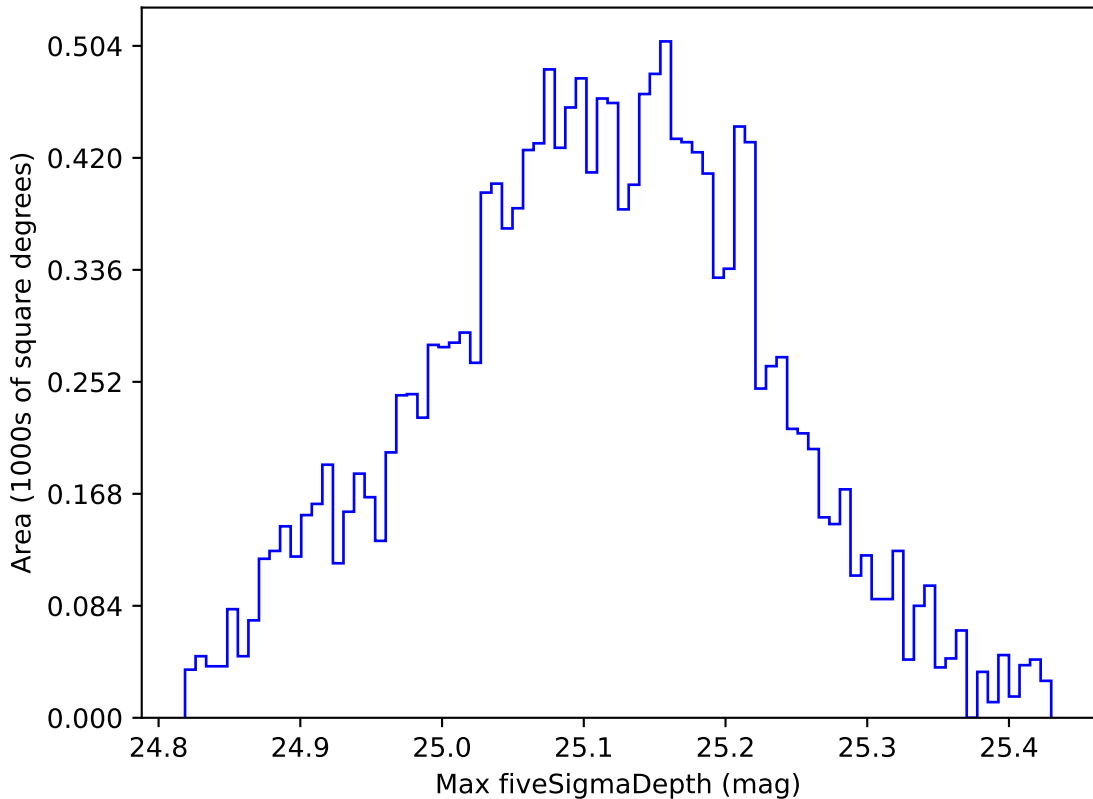
ddf_acor_sf10_lsf15_lsr20_v3.4_10yrs WFD all bands: Max fiveSigmaDepth
