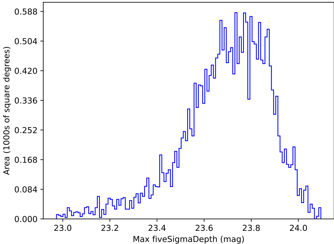
ddf_acor_sf10_ls15_lsr20_v3.4_10yrs All sky u band: Max fiveSigmaDepth
