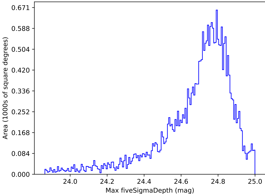
ddf_acor_sf10_lsf15_lsr20_v3.4_10yrs All sky r band: Max fiveSigmaDepth
