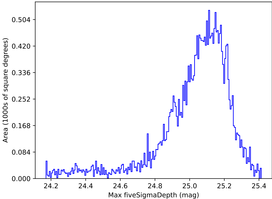
ddf_acor_sf10_ls15_lsr20_v3.4_10yrs All sky g band: Max fiveSigmaDepth
