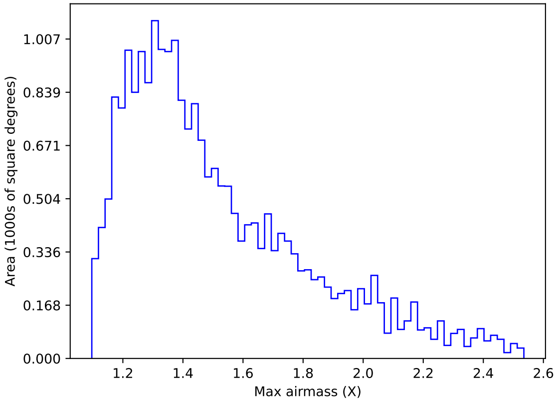
ddf_acor_sf10_lsf15_lsr20_v3.4_10yrs Yr 1 u band: Max airmass
