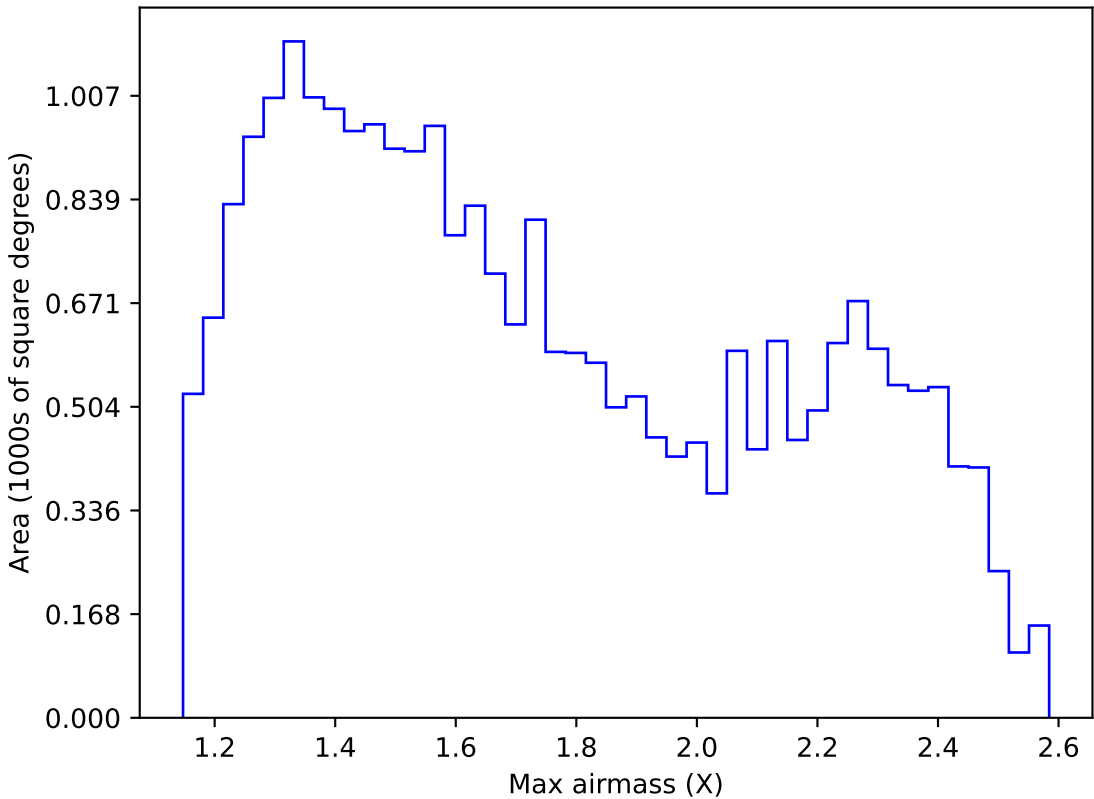
ddf_acor_sf10_ls15_lsr20_v3.4_10yrs Yr 1 r band: Max airmass
