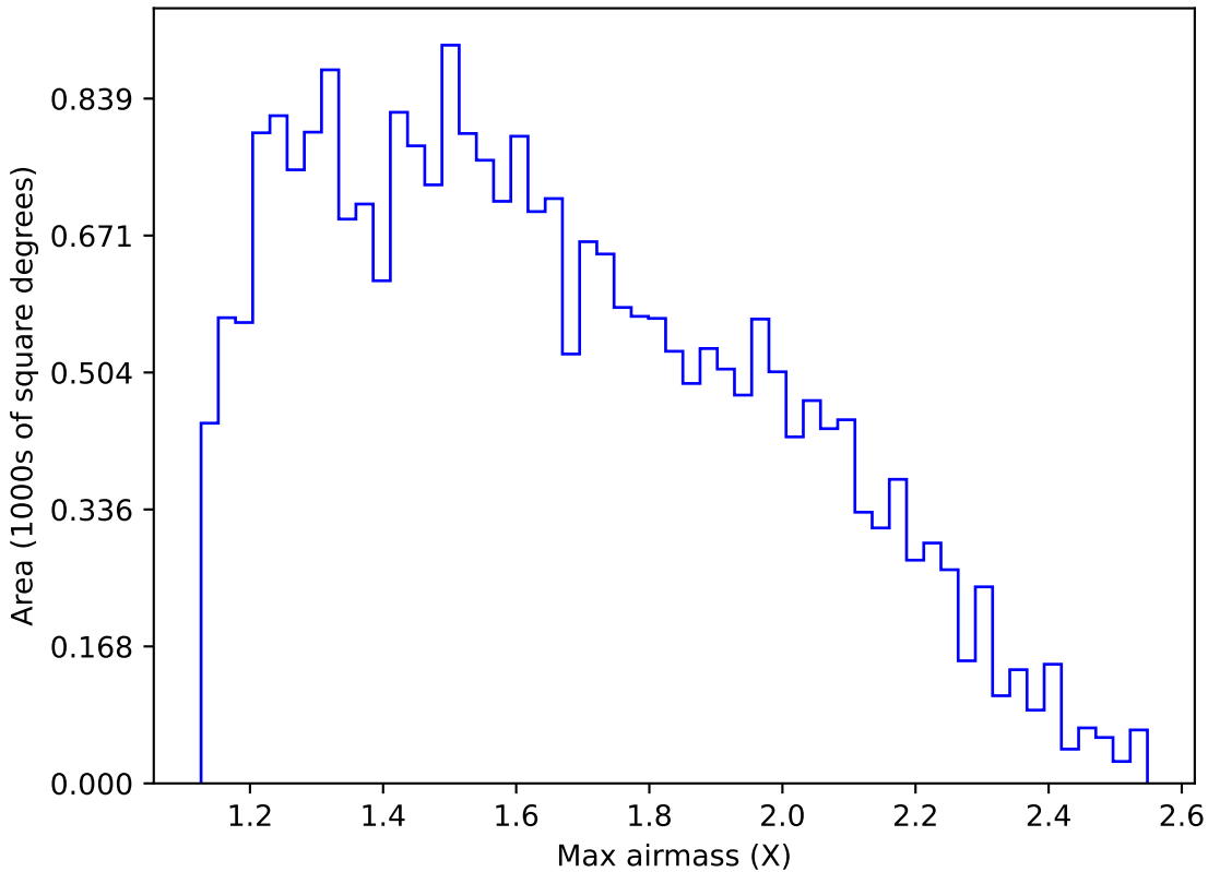
ddf_acor_sf10_lsf15_lsr20_v3.4_10yrs Yr 1 g band: Max airmass
