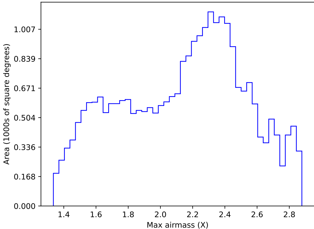
ddf_acor_sf10_lsf15_lsr20_v3.4_10yrs Yr 1 all bands: Max airmass
