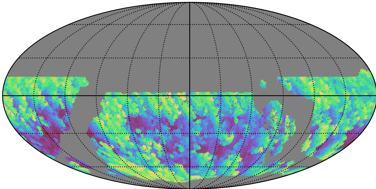
ddf_acor_sf10_lsf15_lsr20_v3.4_10yrs WFD y band: Max airmass
