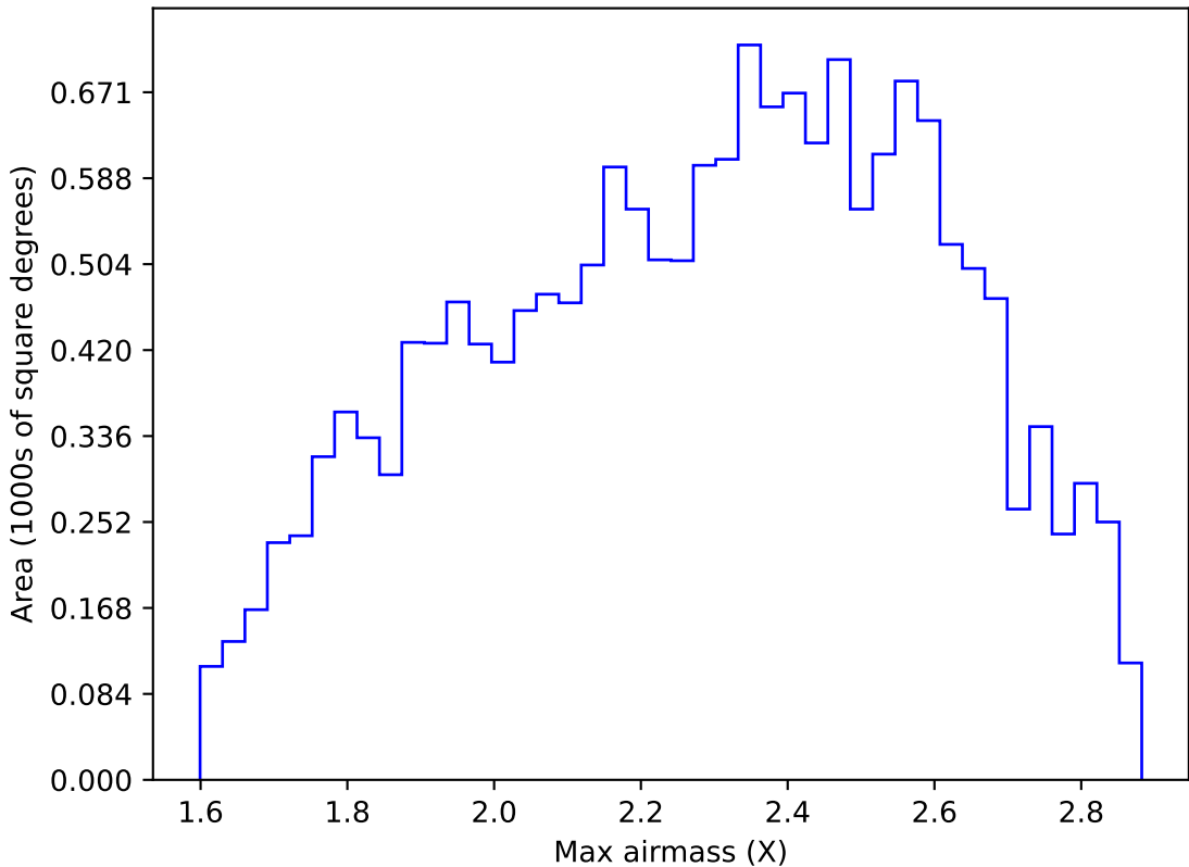
ddf_acor_sf10_ls15_lsr20_v3.4_10yrs WFD y band: Max airmass
