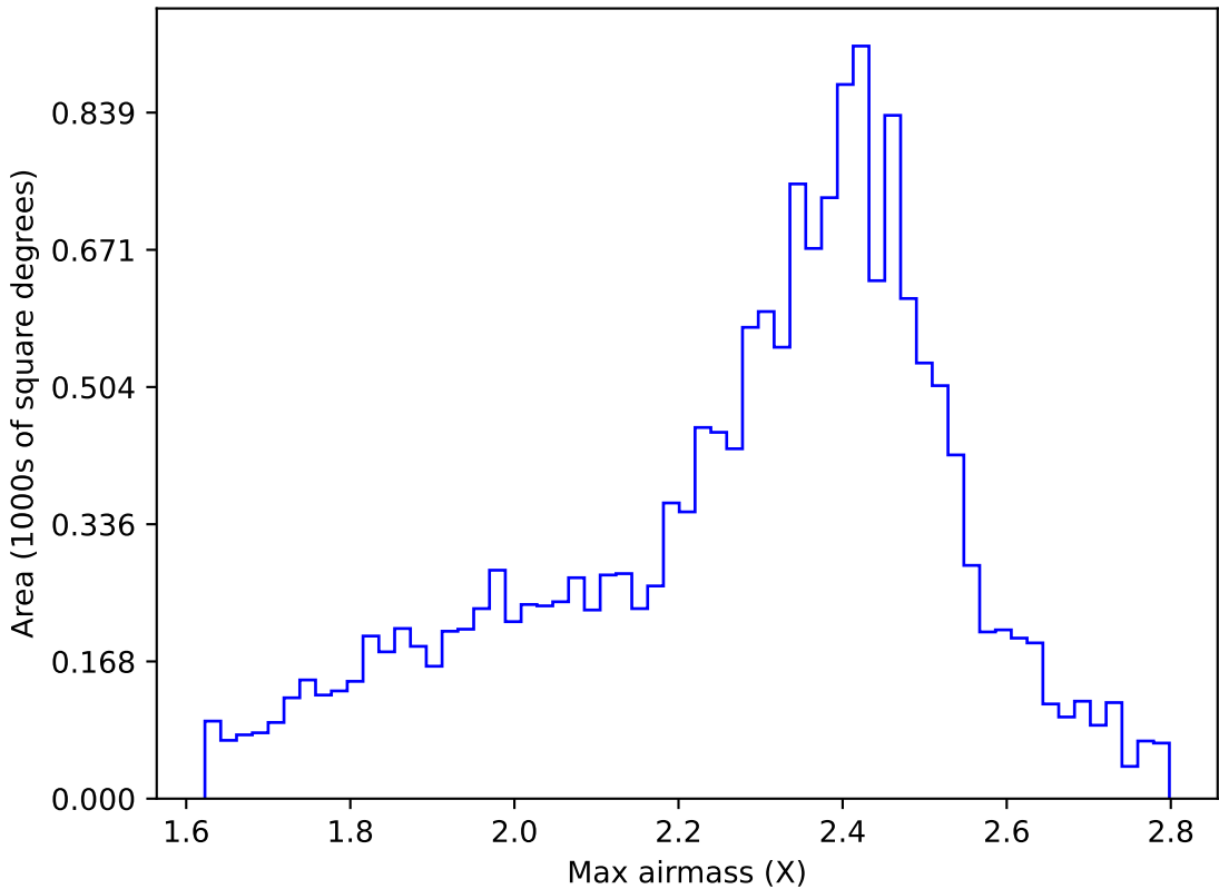
ddf_acor_sf10_ls15_lsr20_v3.4_10yrs WFD r band: Max airmass
