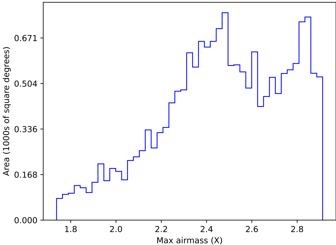
ddf_acor_sf10_lsf15_lsr20_v3.4_10yrs WFD i band: Max airmass
