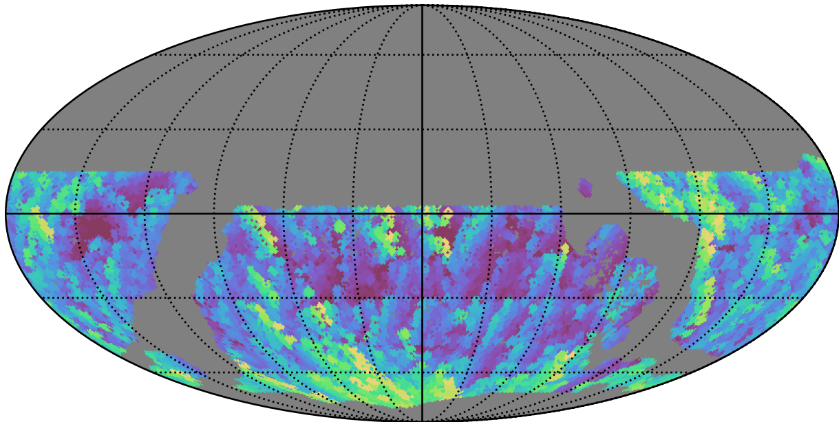
ddf_acor_sf10_lsf15_lsr20_v3.4_10yrs WFD g band: Max airmass
