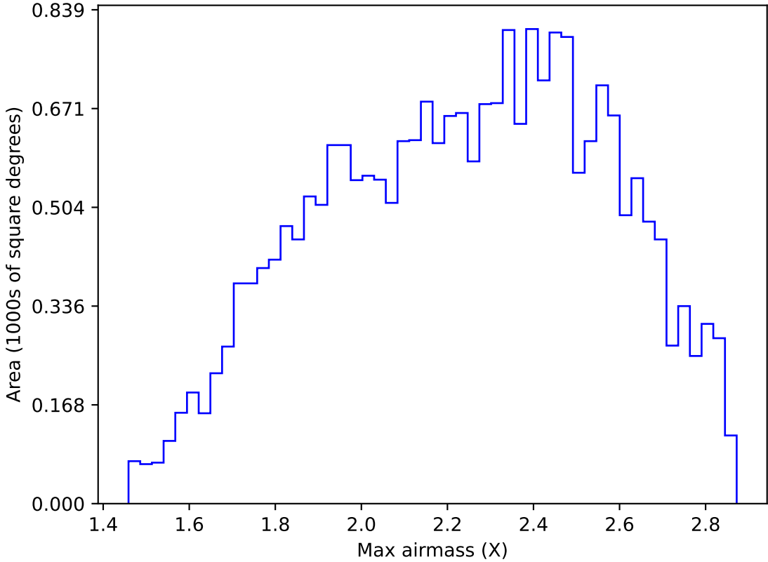
ddf_acor_sf10_lsf15_lsr20_v3.4_10yrs All sky y band: Max airmass
