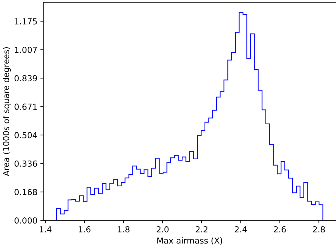
ddf_acor_sf10_lsf15_lsr20_v3.4_10yrs All sky r band: Max airmass
