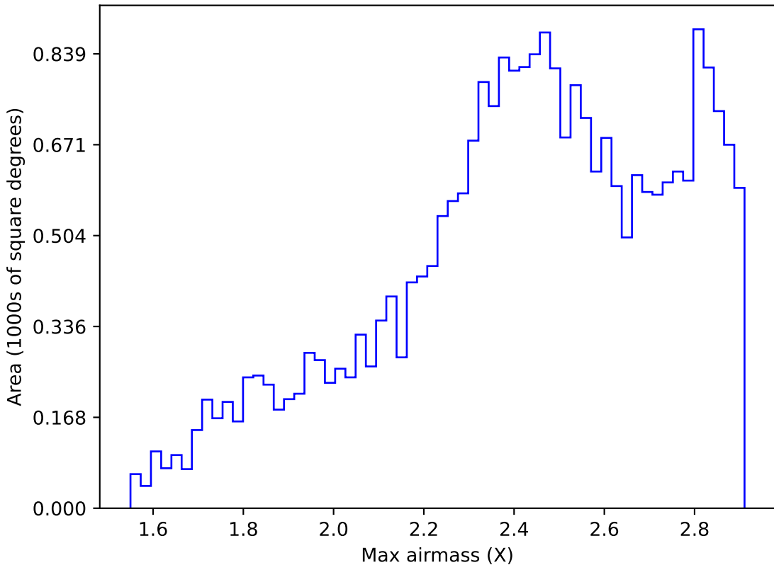
ddf_acor_sf10_lsf15_lsr20_v3.4_10yrs All sky i band: Max airmass
