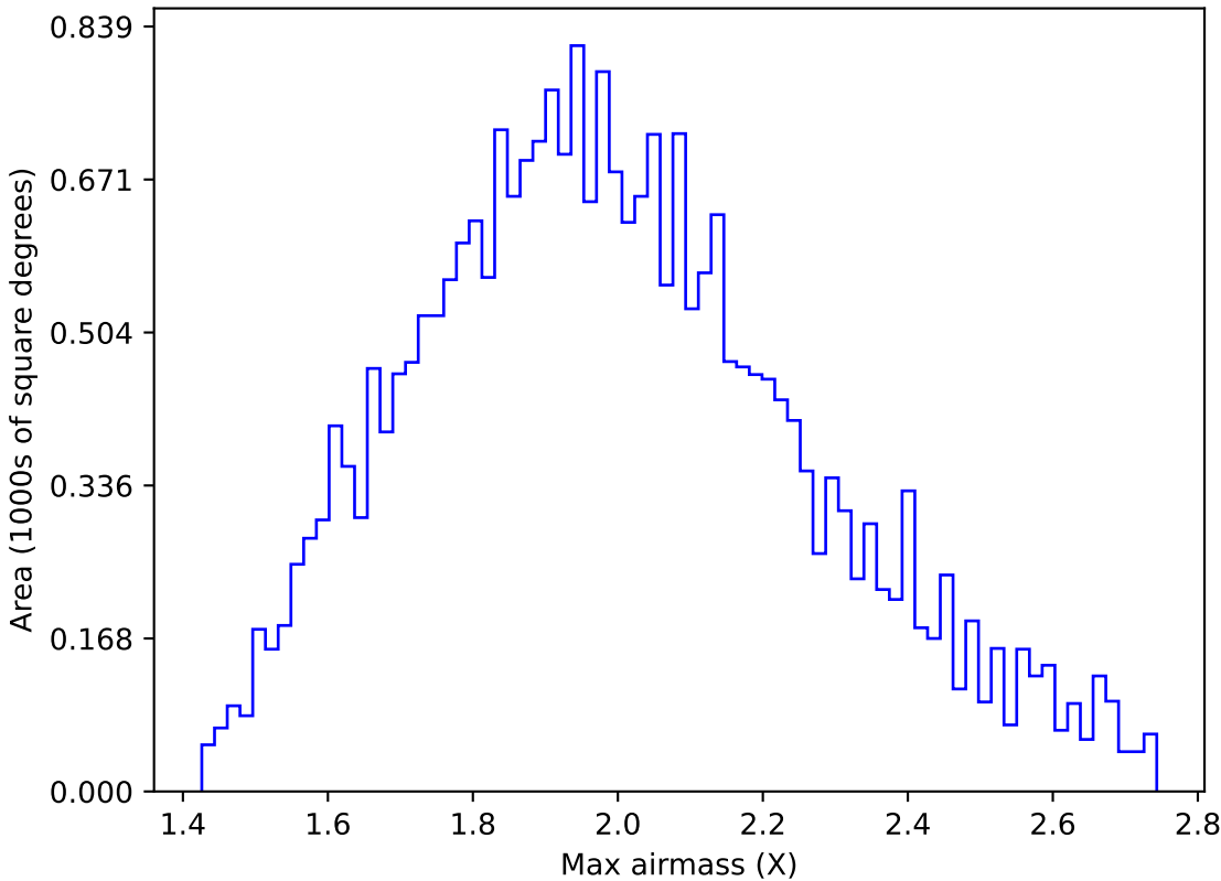
ddf_acor_sf10_lsf15_lsr20_v3.4_10yrs All sky g band: Max airmass
